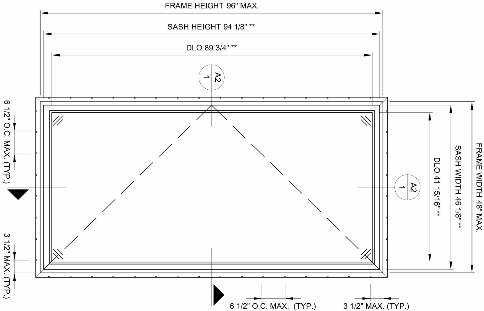
A1 ELEVATION 1 SCALE 1:1
